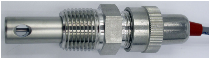
AST51 sensor with 1/2" MNPT 316SS compression fitting rated to 500 psig shown in the K=1.0/cm cell constant configuration.
